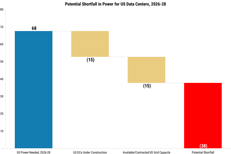
Exhibit 7: We Project a 38GW Power Shortfall in 2026-2028.
